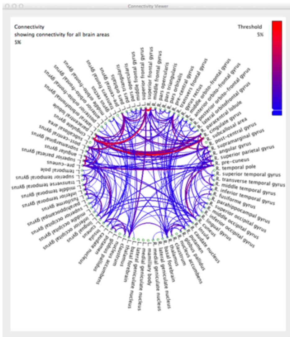
Fig. 2: The BrainSuite13 Connectivity Viewer tool, which visualizes the connectivity matrix computed from the data shown in Fig. 1. This view is synchronized with the main window and can be used to select fiber tracts that are connected to specific labeled ROIs.
